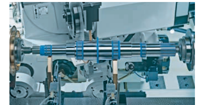
OD grinding with QUICKPOINT
